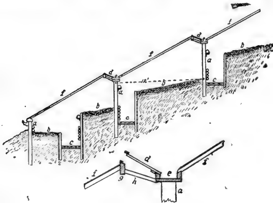
FIG. 8. SIDEHILL HOUSES ( Section ).
